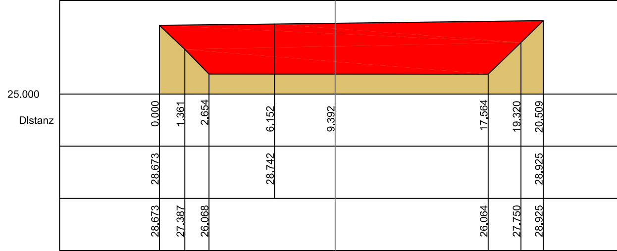
Profil 3 - 3' Station 51.16 m - Fläche -48.28 m 2
