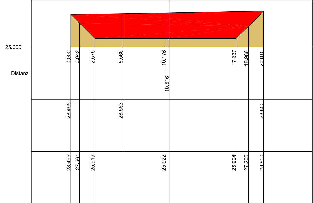
Profil 6 - 6' Station 135.53 m - Fläche -55.86 m 2
