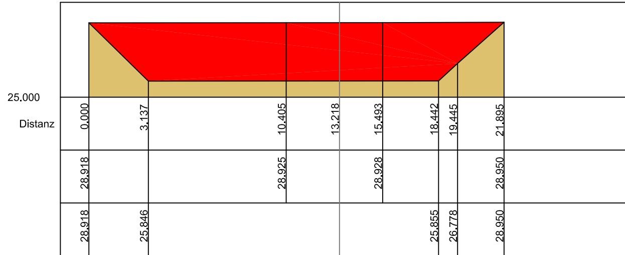
Profil 7 - 7' Station 170.19 m - Fläche -73.61 m 2
