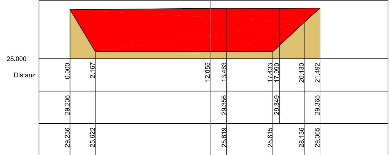
Profil 8 - 8' Station 199.68 m - Fläche -67.91 m 2
