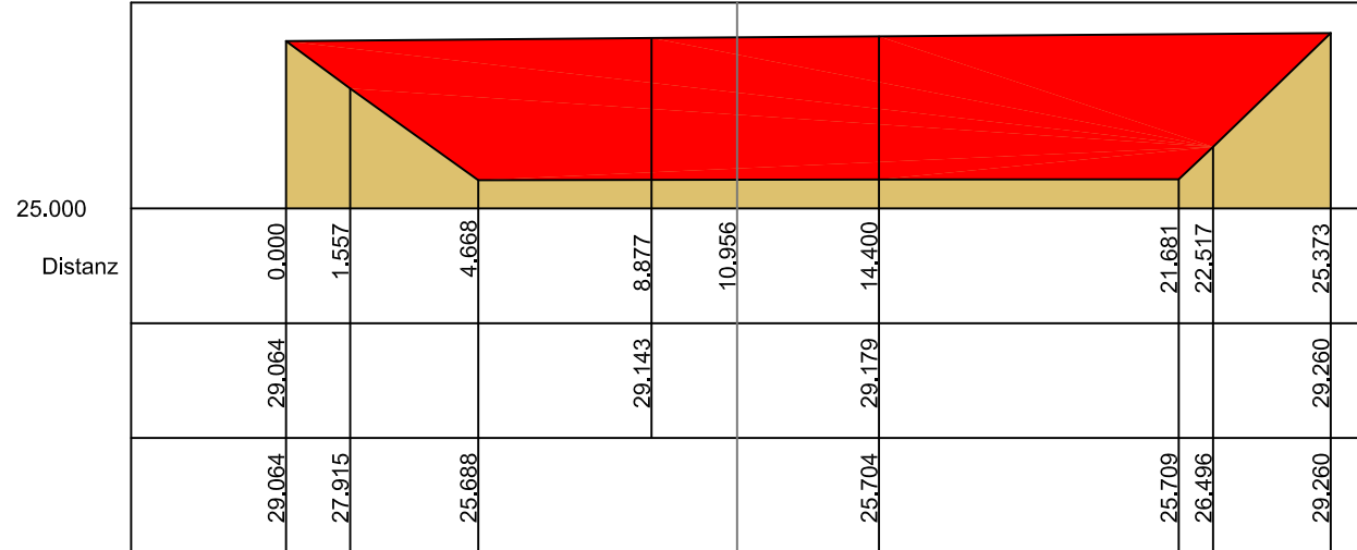
Profil 9 - 9' Station 208.02 m - Fläche -5.05 m 2
