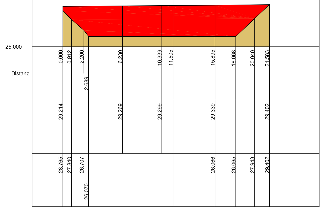
Profil 4 - 4' Station 94.03 m - Fläche -48.82 m 2
